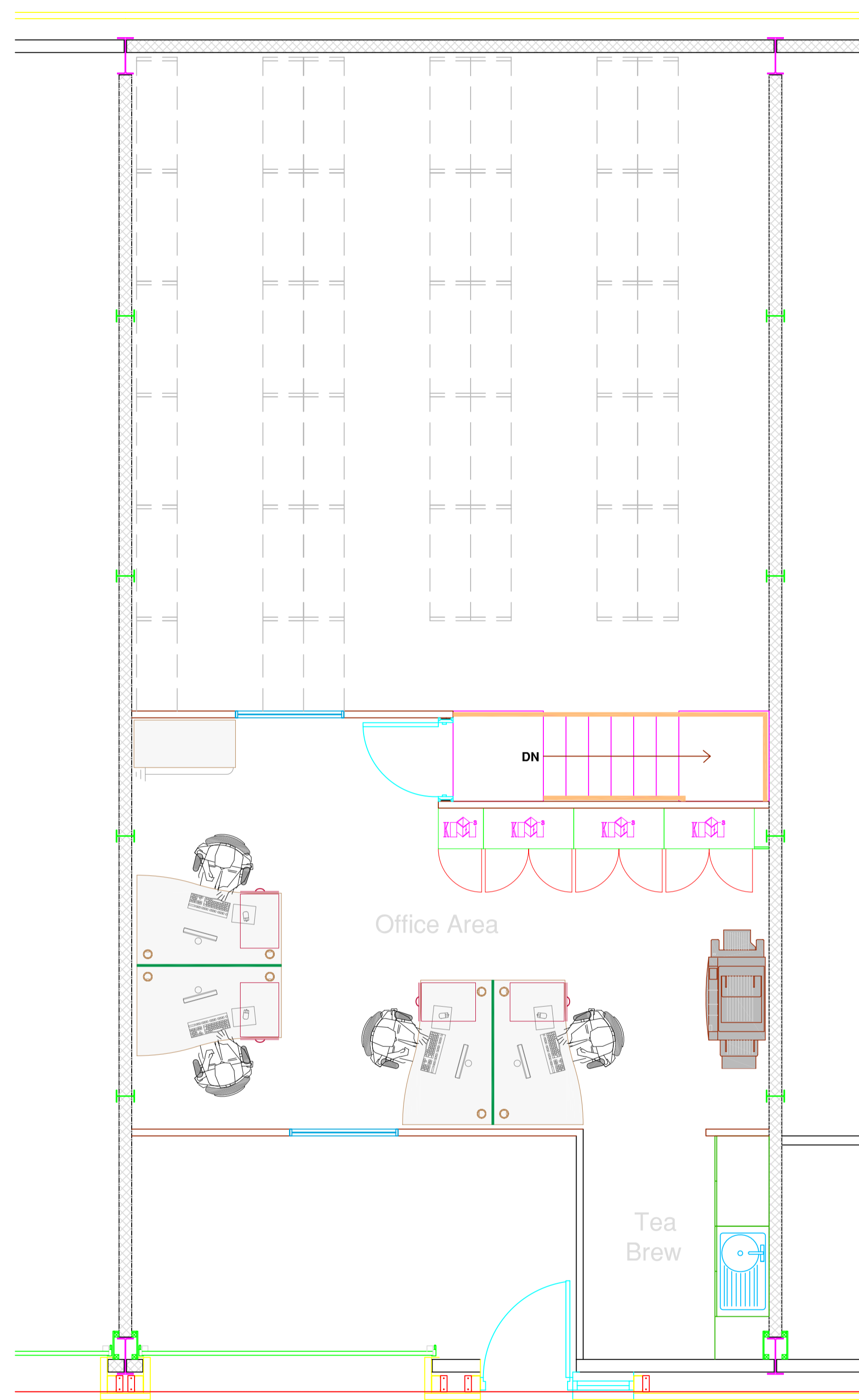
Unit 7 Mezz Floor Layout
